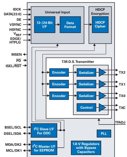
TFP510 block diagram.
