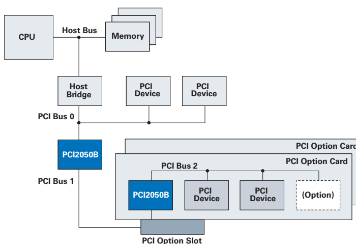
Typical PCI-to-PCI bridge system application.
